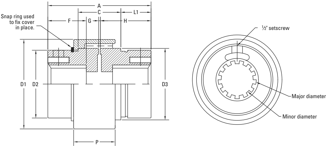
Fig. 35. Quick-Flex splined hubs.
