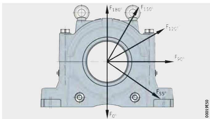
Figure 13 Load directions F for guide values for housing rupture load and maximum load carrying capacity of connecting screws
