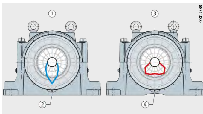
Figure 1 Influence of housing design on the load distribution in the bearing
