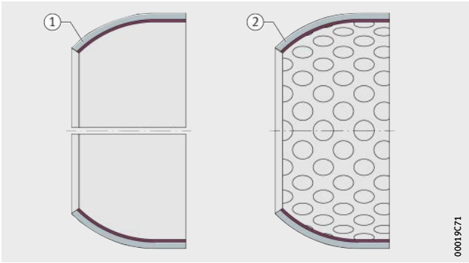
Figure 2 Ball cups
