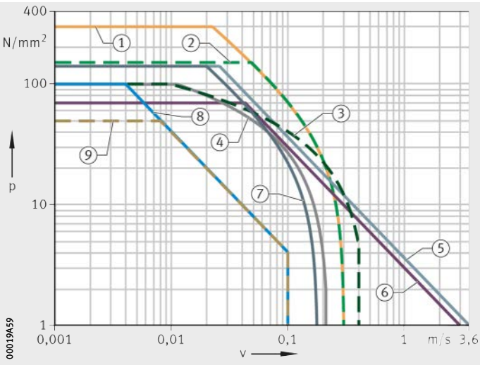
Figure 2 pv diagram
