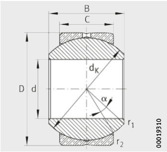
GE..-PB Steel/bronze
