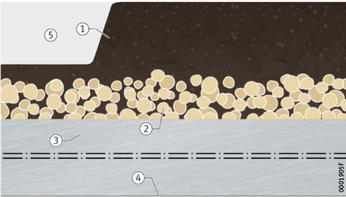
Figure 1 Low-maintenance plain bearing material E50
