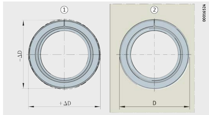
Figure 3 Out of roundness and roundness
