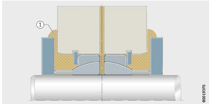
Figure 6 Sealing by means of grease collar
