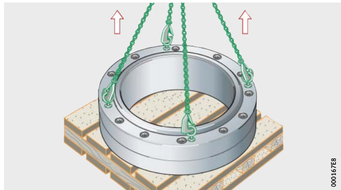
Figure 1 Transport by means of eye bolts
