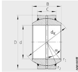
GE..-FO-2TS Steel/steel
