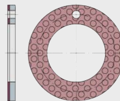
EGW..-E50
