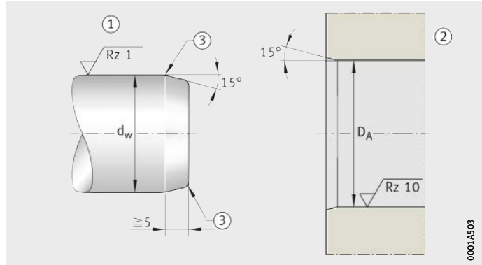
Figure 4 Design of adjacent components
