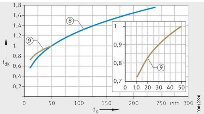
Figure 22 Correction factor for sphere diameter
