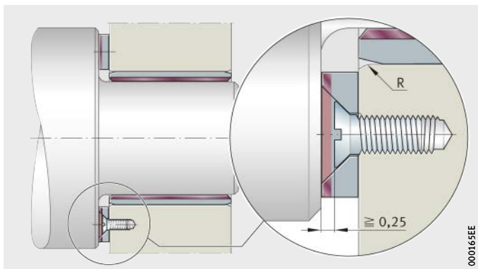
Figure 12 Prevention of rotation by countersunk head screw
