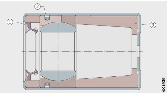
Figure 8 Prop shaft centring bearing
