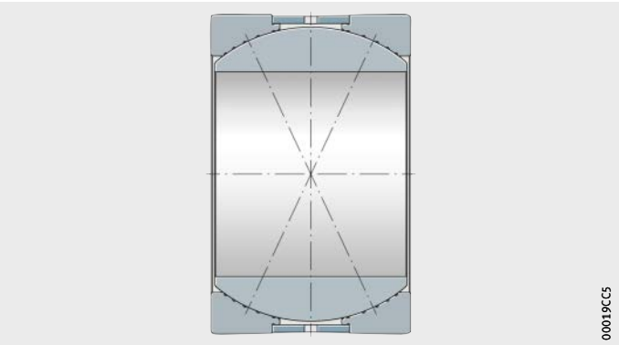
Figure 7 Locating bearing for articulated frame steering system
