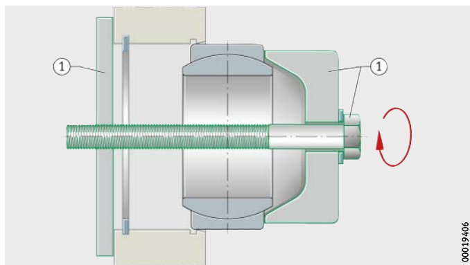
Figure 4 Special mounting equipment for larger bearings
