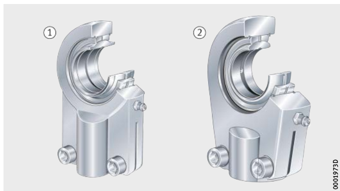
Figure 3 Hydraulic rod ends with thread clamping device
