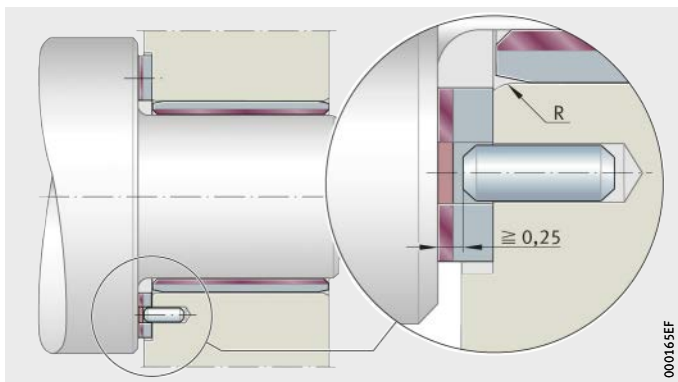
Figure 11 Prevention of rotation by dowel pin
