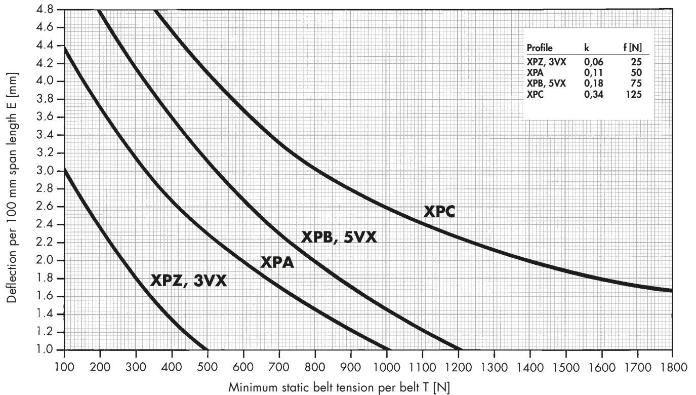
Diagram 10: Belt tension characteristics for optibelt X-POWER M=S wedge belts – raw edged, moulded coggd
