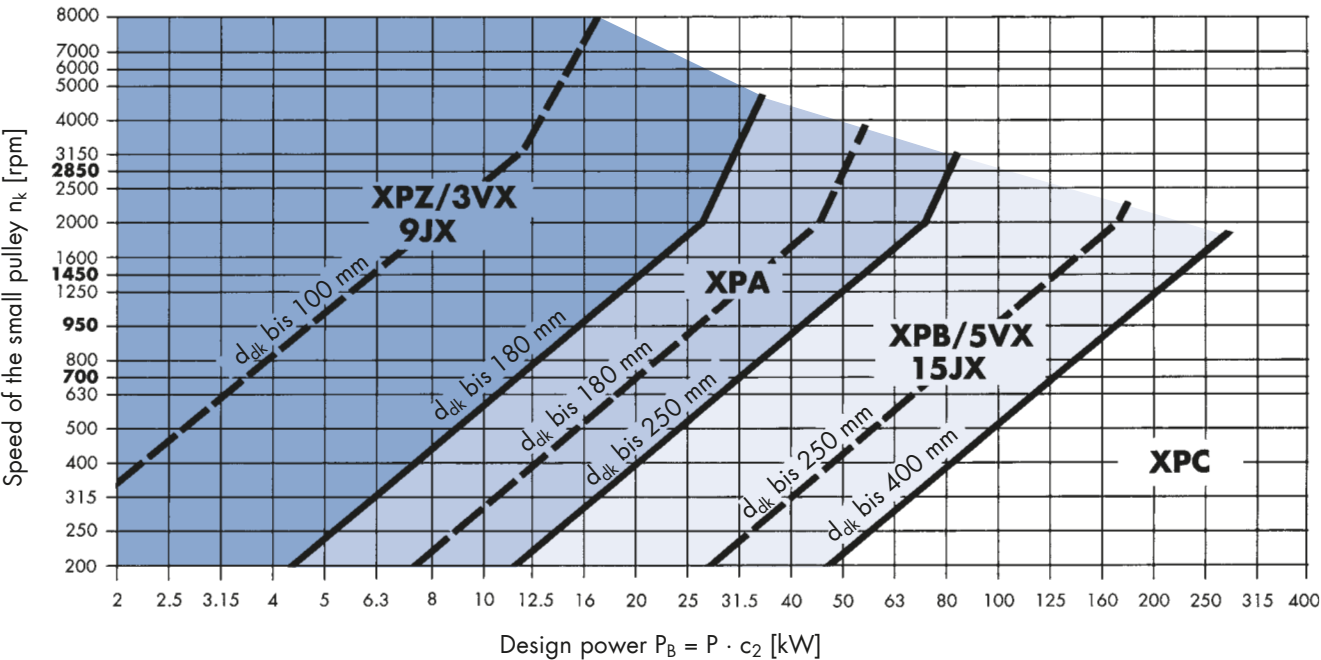
Diagram 4: optibelt SUPER X-POWER M=S wedge belts
